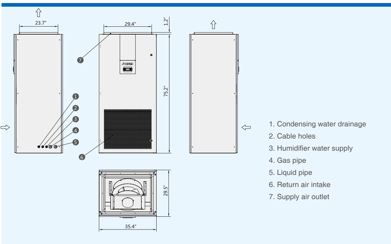
C2 Top throw (air) unit dimensions
