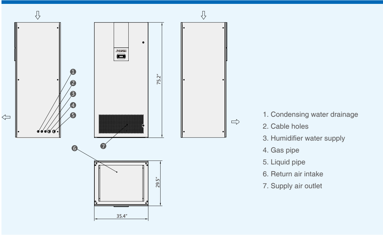
C2 Replacement (air) unit dimension drawing
